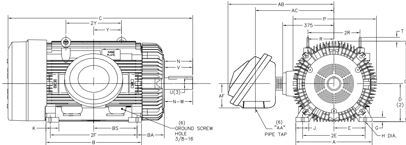
DIMENSIONS ARE IN MILLIMETERS; SEE SHEET 1 FOR DIMENSIONS IN INCHES
